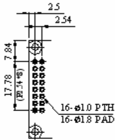
PIN DETAIL
